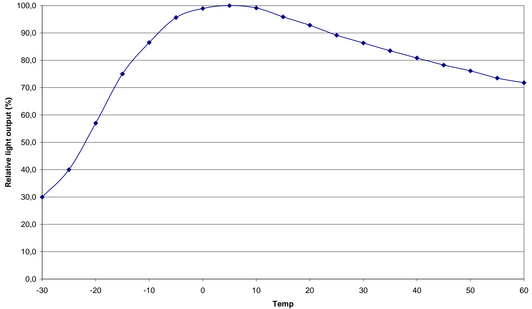
Relative Light Output as a Function of Temperature Aura LL 58 W Thermo
